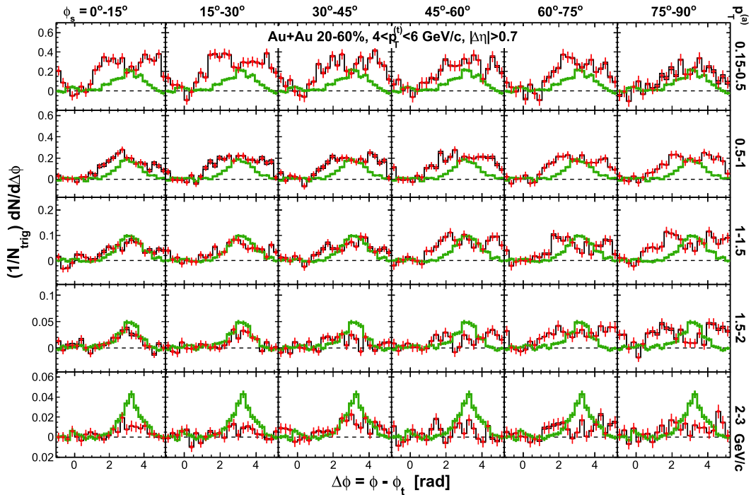
Fig. C14. (color online) Same as in Fig. C13 but for trigger particle 4 < p_T^{(a)} < 6 GeV/c.
