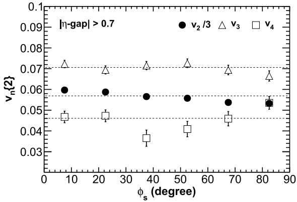
Fig. 23. (color online) Harmonic v_n\{p_T - p_T\} of associated particles of 1.5 < p_T^{(a)} < 2 GeV/c as a function of \phi_s of trigger particles of 3 < p_T^{(i)} < 4 GeV/c. Note that v_2\{p_T - p_T\} is scaled down by a factor of 3 to fit into the plot coordinate range. v_n\{p_T - p_T\} is measured by the two-particle cumulant method with particle pairs from the same associated p_T^{(a)} bin and with \eta_{\text{gap}} = 0.7 . The data are from minimum-bias 20%-60% Au+Au collisions. Error bars are statistical. The horizontal lines are to guide the eye.
