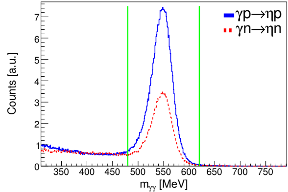
Fig. 2. Invariant mass histogram of two photons after the missing mass and the coplanarity cut: Solid line: for the quasi-free reaction on the proton. Dashed line: for the quasi-free reaction on the neutron. The green vertical lines denote the invariant mass cut limits to select events with an \eta -meson.
