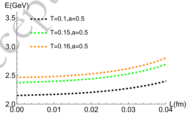
Fig. 8. (color online) The potential energy E of the \Sigma_u^- state as a function of L for a = 0.5 . The curves represent temperatures of 0.1 GeV (black dashed), 0.15 GeV (green dashed), and 0.16 GeV (orange dashed).
