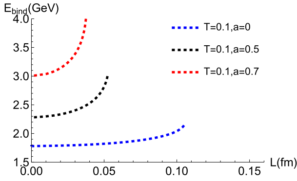
Fig. 6. (color online) Evolution of the binding energy of the \Sigma_u^- state as a function of the separation L at T = 0.1 \text{ GeV} . Dashed blue, black, and red curves represent anisotropy values a = 0, 0.5, and 0.7, respectively.
