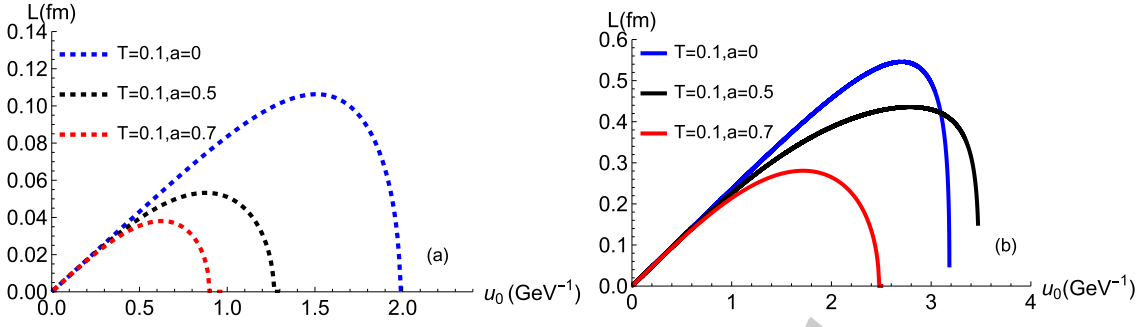
Fig. 4. (color online) Dependence of the separation distance on u_0 for the \Sigma_g^+ and \Sigma_u^- channels at T = 0.1 \text{ GeV} and for different values of the anisotropy parameter a . (a) \Sigma_u^- : Dashed blue, black, and red curves correspond to anisotropy parameters a = 0, 0.5, and 0.7, respectively. (b) \Sigma_g^+ : Solid blue, black, and red curves correspond to anisotropy parameters a = 0, 0.5, and 0.7, respectively.
