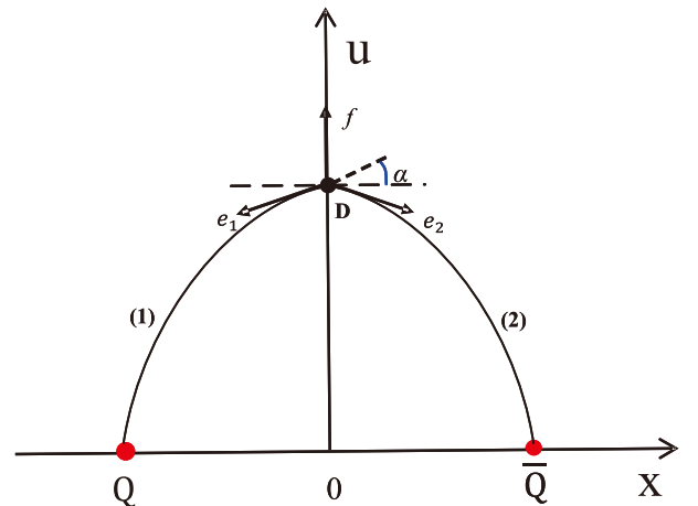
Fig. 1. (color online) Geometric setup of the hybrid meson model [75]. The quark and antiquark are shown as red markers along the x -axis, whereas the holographic defect is represented by a black symbol on the u -axis. The black lines connecting the defect to the quarks represent fundamental strings. The quantities e_1 and e_2 denote the tensions of strings (1) and (2), respectively. The angle between string (1) and the x -axis is denoted by \alpha .
