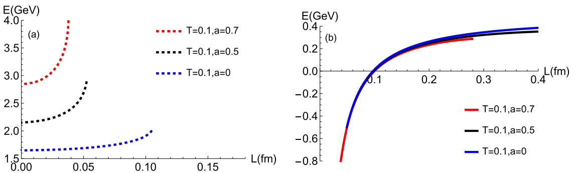
Fig. 5. (color online) Behavior of the static potential for the \Sigma_u^- (a) and \Sigma_g^+ (b) channels as a function of the separation L at T = 0.1 \text{ GeV} . (a) In the \Sigma_u^- channel, the dashed curves correspond to anisotropy parameters a = 0 (blue), 0.5 (black), and 0.7 (red). (b) In the \Sigma_g^+ channel, the solid curves follow the same color scheme for the corresponding a values.
