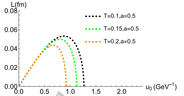
Fig. 7. (color online) Separation distance L as a function of the bulk turning point u_0 ( a = 0.5 ). The black, green, and orange dashed lines correspond to thermal scales of 0.1, 0.15, and 0.2 GeV, respectively.
