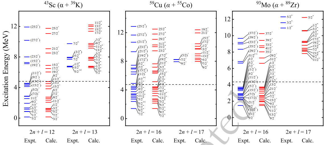
Fig. 3. (color online) The comparisons of the calculated doublet parity bands with the available candidates [50] for \alpha -cluster states in heavier nuclei, where the dash lines denote the \alpha -cluster thresholds. The intrinsic spins of ^{39}\text{K} , ^{55}\text{Co} and ^{89}\text{Zr} are 3/2^+ , 7/2^- and 9/2^- , respectively.
