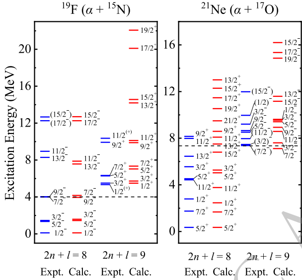
Fig. 1. (color online) The comparisons of the calculated parity doublet bands of 2n + l = 8 and 9 for \alpha -cluster states in ^{19}\text{F} ( \alpha + ^{15}\text{N} ) and ^{21}\text{Ne} ( \alpha + ^{17}\text{O} ) with the experimental data [20, 42, 50], where the dash lines dictate the \alpha -cluster breakup thresholds. The intrinsic spins of ^{15}\text{N} and ^{17}\text{O} are 1/2^- and 5/2^+ , respectively.
