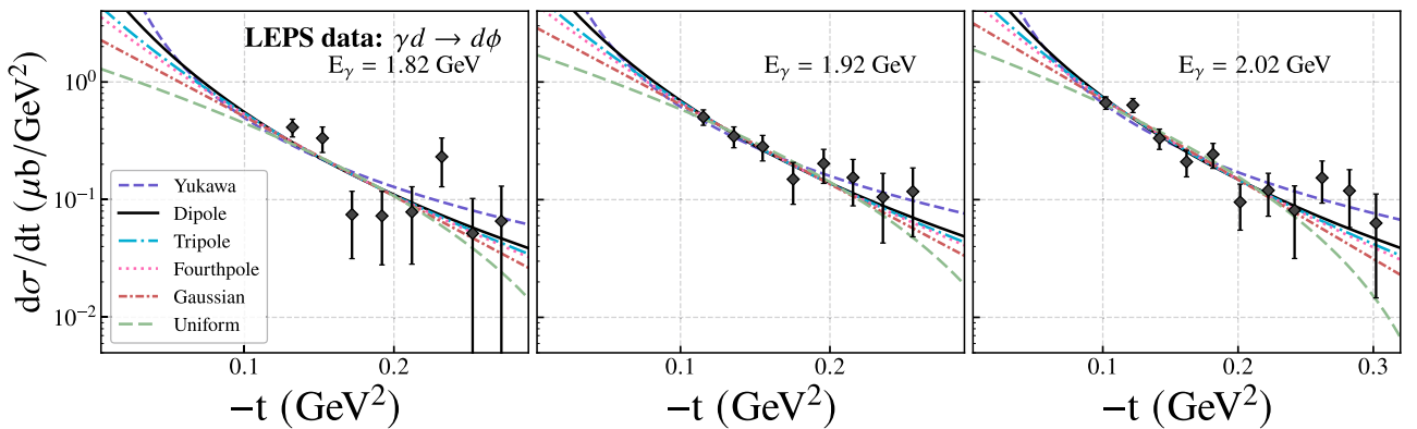
Fig. 4. (color online) Differential cross sections of near-threshold \phi photoproduction measured by the LEPS Collaboration [41, 43], fitted with six model parameterizations.
