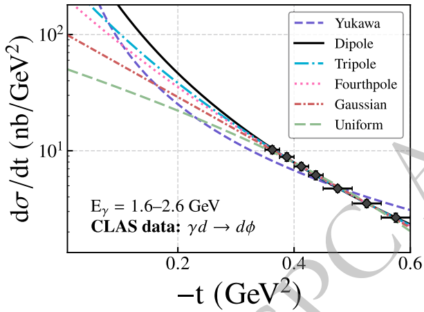
Fig. 3. (color online) Differential cross sections of near-threshold \phi photoproduction measured by CLAS [42], fitted with six model parameterizations.
