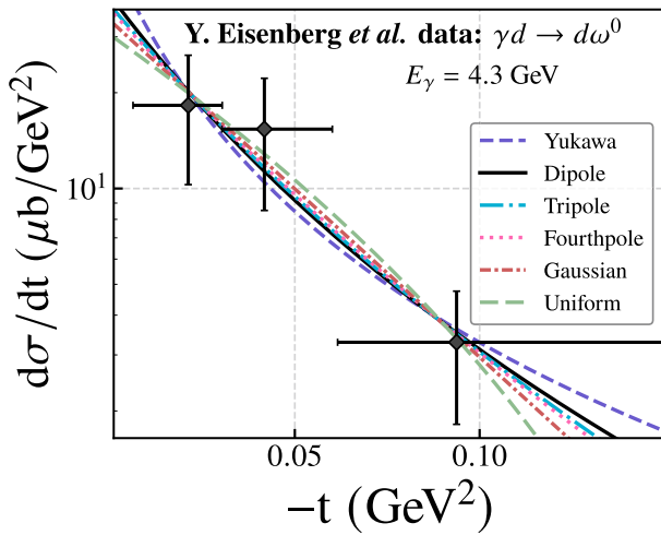
Fig. 2. (color online) Differential cross sections of near-threshold \omega photoproduction measured by Y. Eisenberg et al. [37], fitted with six models.
