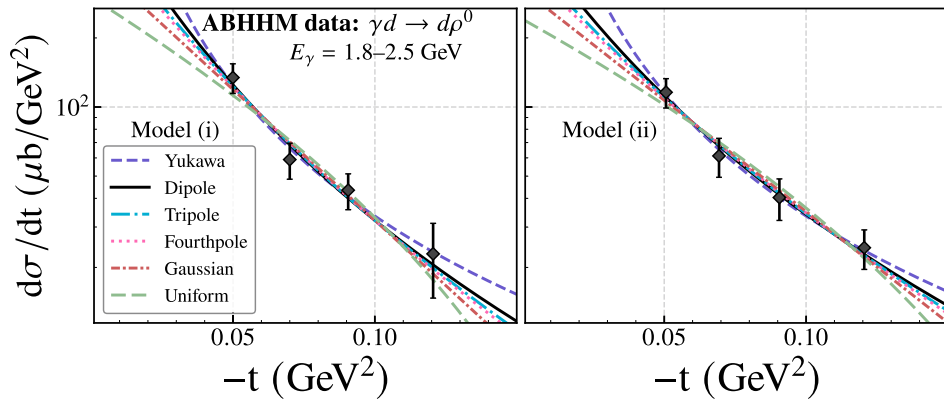
Fig. 1. (color online) Differential cross sections of near-threshold \rho^0 photoproduction on deuteron fitted with six models using two resonance schemes (Model i and Model ii) from ABHHM Collaboration data [36].
