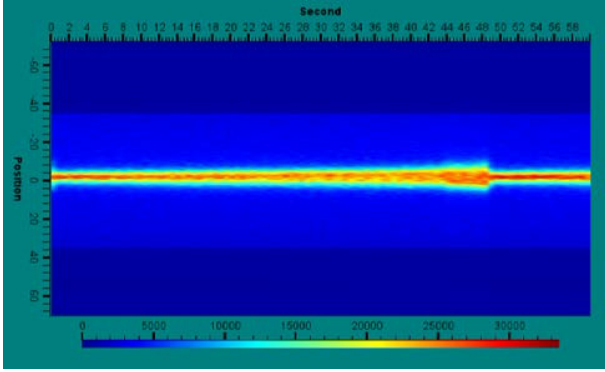
Fig. 3. (color online) Stored ^{56}\text{Fe}^{26+} at 25 MeV/n at CSRe (corresponding to a magnetic rigidity of 1.5 Tm) [13]
