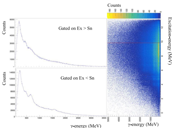
Fig. 2. (color online) \gamma -rays in coincidence with protons from the ^{85}\text{Kr}(d, p\gamma)^{86}\text{Kr} reaction at 10 MeV/u [9]. Right: \gamma -energy versus total excitation energy. Left: gamma spectra gated above (up) and below (down) the neutron binding energy ( S_n=9.86 MeV). The 2^+ and 4^+ excitations in ^{86}\text{Kr} are clearly visible.
