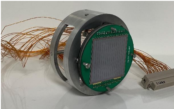
Fig. 4. (color online) Si strip detector for proton inelastic scattering experiments (three layers with the thicknesses of 300, 500, and 500 \mu\text{m} ) [14, 15]
