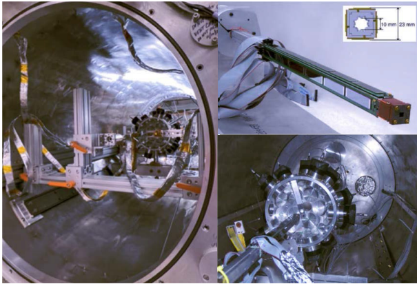
Fig. 1. (color online) HELIOS spectrometer and the Apollo array at the ATLAS facility in Argonne (USA) [10].
