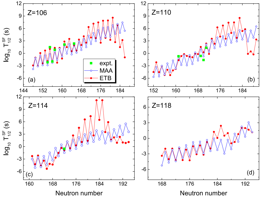
Fig. 7. (color online) Same as Fig. 6 but for Sg, Ds, Fl, and Og isotopes.
