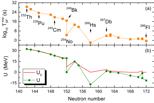
Fig. 2. (color online) (a) Maximum measured value of \log_{10} T_{SF} in each isotopic chain with mass numbers from A = 232 to A = 286 . (b) Corresponding values of the effective tunneling barrier U . The red curve denotes the relative barrier height U_0 = V_{top} - Q_{sf} + \Delta .
