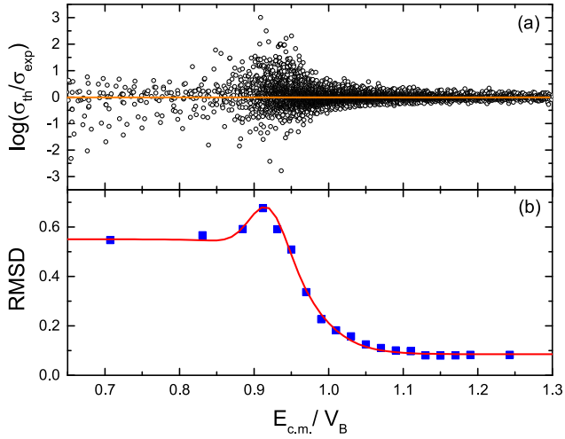
Fig. 6. (color online) (a) Deviations between predicted capture cross sections with EBD2.2 and experimental data as a function of the ratio E_{\text{c.m.}}/V_B . (b) Root-mean-square deviations with respect to the measured capture cross sections (in log) as a function of E_{\text{c.m.}}/V_B . The squares denote the calculated results with the data in (a). The solid curve denotes the results by fitting the squares.
