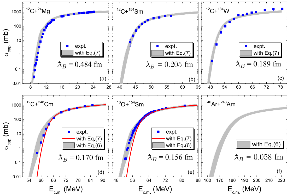
Fig. 7. (color online) Fusion excitation functions for six fusion reactions with deformed nuclei. The shadow represents the uncertainty of EBD2.2 predictions, and the squares represent the experimental data taken from Refs. [6, 54–58].
