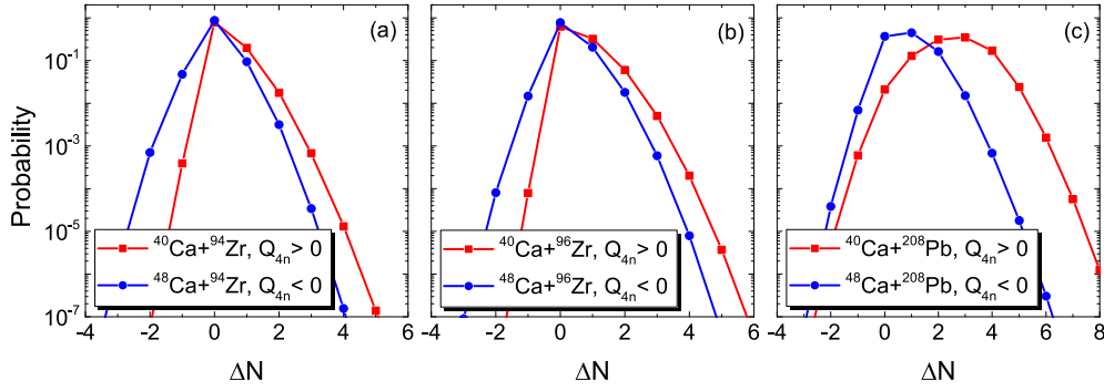
Fig. 8. (color online) Neutron transfer probability as a function of the number of neutrons transferred from the target nucleus to the projectile nucleus in the back-angle quasi-elastic scattering of ^{40}\text{Ca}+^{94,96}\text{Zr} and ^{40}\text{Ca}+^{208}\text{Pb} . The squares and circles indicate the results for reactions with Q_{4n} > 0 and those with Q_{4n} < 0 , respectively.
