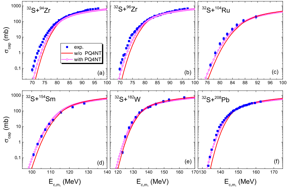
Fig. 4. (color online) Same as Fig. 3 but for reactions ^{32}\text{S}+^{94}\text{Zr} [45], ^{32}\text{S}+^{96}\text{Zr} [46], ^{32}\text{S}+^{104}\text{Ru} [47], ^{32}\text{S}+^{154}\text{Sm} [38], ^{32}\text{S}+^{182}\text{W} [48], and ^{32}\text{S}+^{208}\text{Pb} [49].
