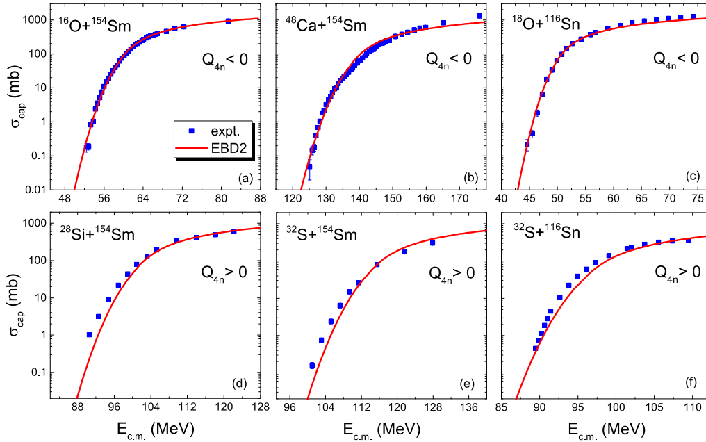
Fig. 1. (color online) Capture excitation functions for ^{16}\text{O} + ^{154}\text{Sm} [6], ^{48}\text{Ca} + ^{154}\text{Sm} [36], ^{18}\text{O} + ^{116}\text{Sn} [26], ^{28}\text{Si} + ^{154}\text{Sm} [37], ^{32}\text{S} + ^{154}\text{Sm} [38], and ^{32}\text{S} + ^{116}\text{Sn} [39]. The squares and curves denote the experimental data and predictions of EBD2 [32], respectively.
