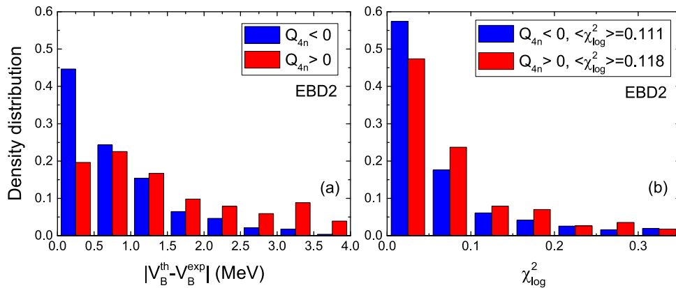
Fig. 2. (color online) (a) Distribution of the discrepancies between the calculated barrier heights V_B^{\text{th}} with EBD2 and extracted ones V_B^{\text{exp}} [40]. (b) Distribution of the mean-square deviation between the predicted cross-sections with EBD2 and the experimental data in logarithmic scale. The blue and red bars denote the results for the cases with Q_{4n} < 0 and Q_{4n} > 0 , respectively.
