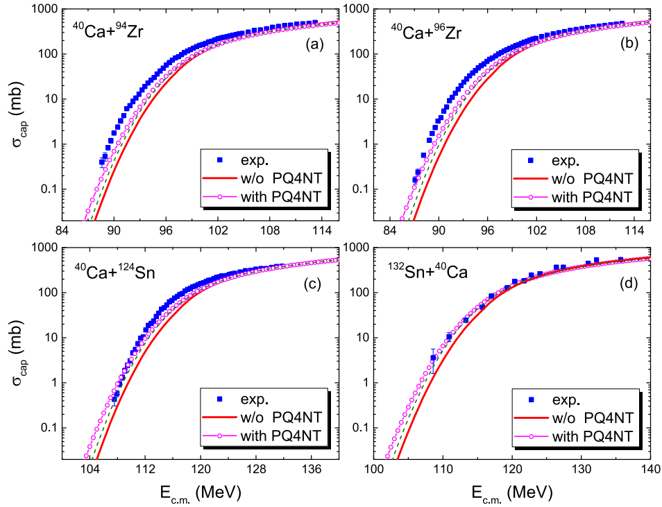
Fig. 3. (color online) Capture excitation functions for reactions ^{40}\text{Ca} + ^{94}\text{Zr} [41], ^{40}\text{Ca} + ^{96}\text{Zr} [42], ^{40}\text{Ca} + ^{124}\text{Sn} [43], and ^{132}\text{Sn} + ^{40}\text{Ca} [44]. The squares denote the experimental data. The solid curves and circles represent the results of EBD2 and those with the PQ4NT effect being considered in the calculations, respectively. The dashed curves represent the results obtained considering the \Delta_{tr} term in Eq. (2) and neglecting the \Delta_{tr} term in Eq. (6).
