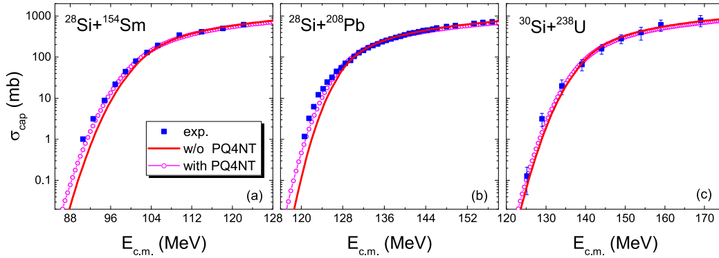
Fig. 5. (color online) Same as Fig. 3 but for reactions ^{28}\text{Si}+^{154}\text{Sm} [37], ^{28}\text{Si}+^{208}\text{Pb} [50], and ^{30}\text{Si}+^{238}\text{U} [51].
