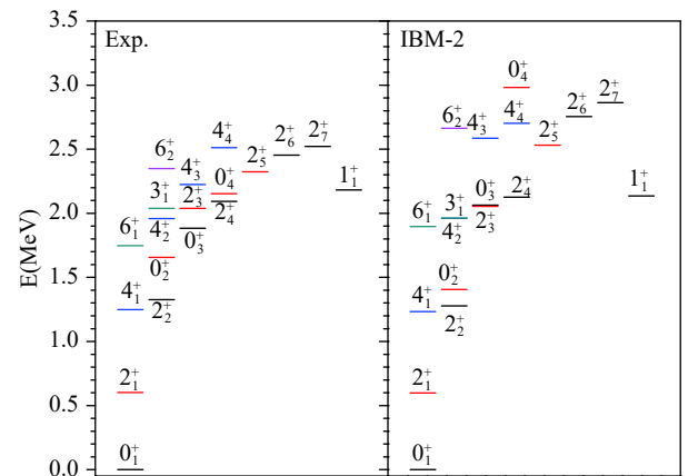
Fig. 1. (color online) Comparison of the calculated and experimental [3, 40] low-lying positive-parity levels of ^{124}\text{Te} .
