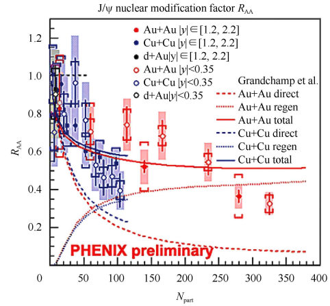
Fig. 3. Nuclear modification factor as a function of a number of participants ( N_{\text{part}} ) for Au+Au and Cu+Cu collisions [21].
