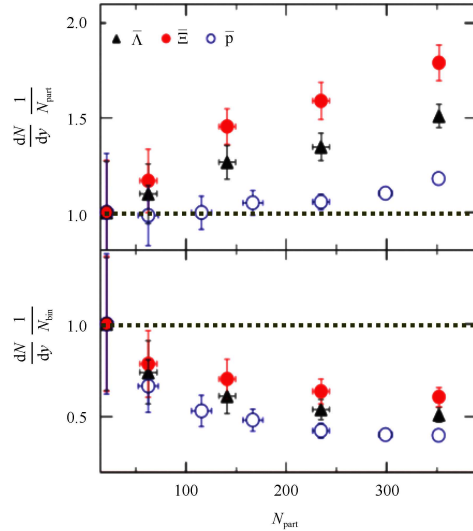
Fig. 2. Yields of some baryons as a function of the centrality (expressed with the number of participants) in Au+Au collisions normalized to the most peripheral point and to number of participant ( N_{\text{part}} ) shown in the upper frame and number of binary collisions ( N_{\text{bin}} ) shown in the lower frame [18]. N_{\text{part}} and N_{\text{bin}} are calculated in the framework of the Glauber model. Different markers with different colors correspond to different baryons as shown.
